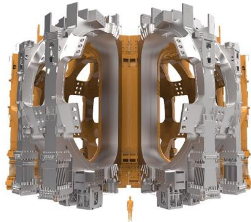
The Toroidal Field Coils, shown in gray
